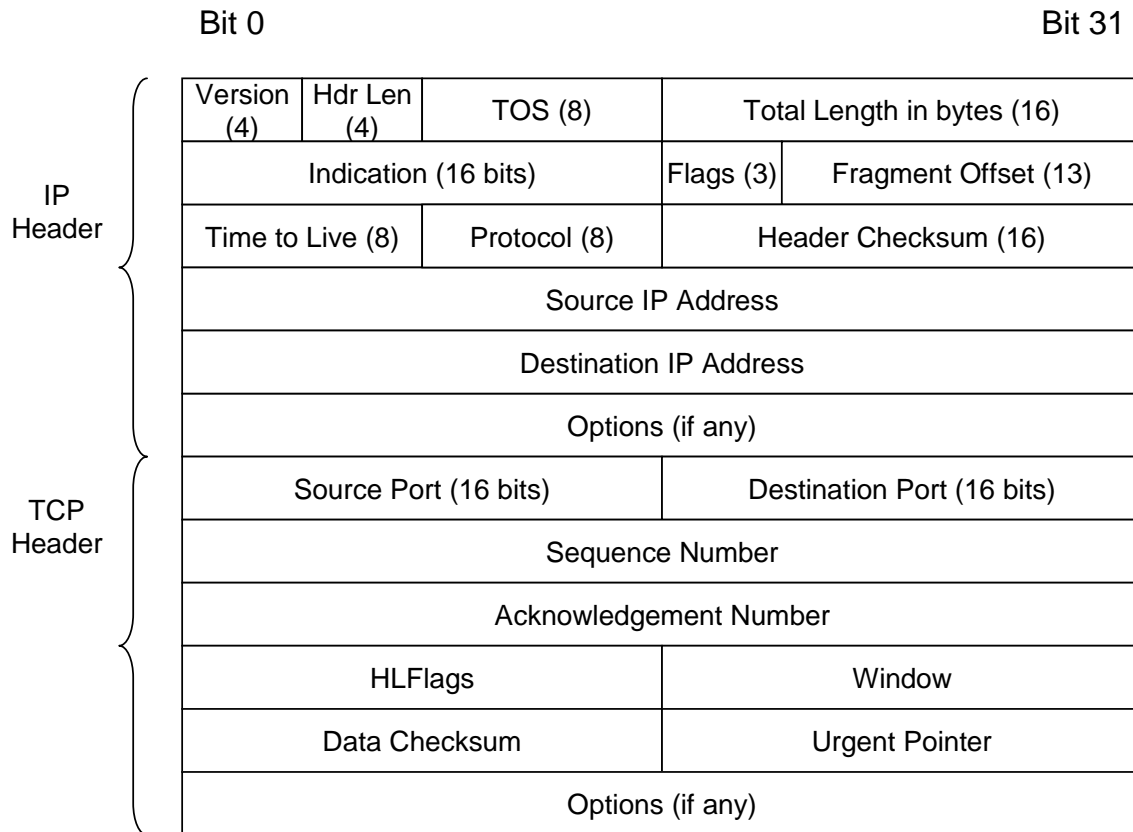
Figure 4. TCP/IP Headers
